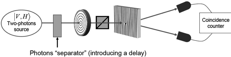
Figure 4. Sketch of the experimental scheme used for generating a biphoton state with OAM correlations and for testing it.
