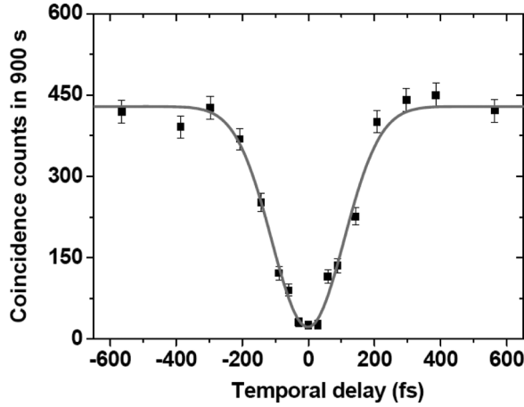
Figure 5. Coincidence counts obtained in the measurement of opposite OAM values for the biphoton generated by the q-plate, as illustrated in Figure 4 [16]. For zero delay the coincidence counts vanish (except for a small background), showing that the OAM of the two photons is fully correlated.
