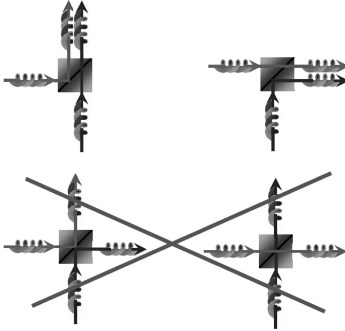
Figure 6. Pictorial illustration of the Hong-Ou-Mandel two-photon interference effect in a beam-splitter for the case of OAM-carrying photons (depicted as little helices). In this example the input OAM of the two photons is opposite, so that if one of the two photon is reflects it is inverted and becomes equal to that of the other photon. It can then be shown that the two processes in the lower panels, leading to exactly the same final state, have opposite amplitudes and cancel (as long as the two photons are otherwise identical). The remaining two processes in the upper panel have a doubled probability of taking place, so that one obtains an enhanced quantum coalescence of the photons in the output ports of the beam-splitter. If the input OAM of the two photon is equal, the interference does not take place because all processes give rise to different outputs and there is no enhancement.
