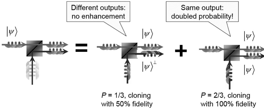
Figure 9. Graphical analysis of the cloning quantum fidelity.
