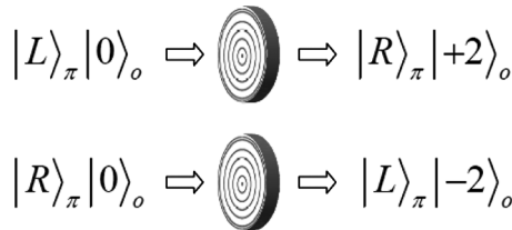
Figure 1. Effect of a q-plate (assumed to be well tuned and having q = 1 ) on a input photon that is in a circular-polarization and zero-OAM quantum state: the spin is inverted and the variation of SAM is entirely converted into OAM, that thus acquires \pm 2\hbar of angular momentum (i.e., the output m = \pm 2 ).
