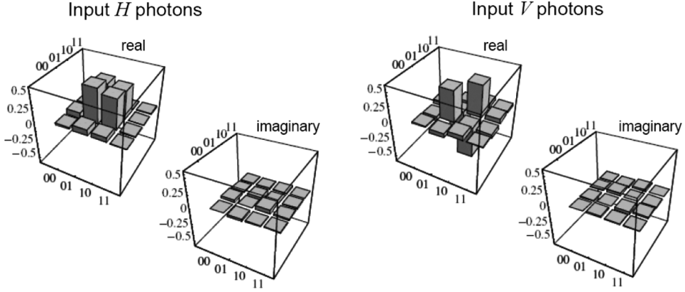
Figure 2. Results of experimental quantum tomography of the photons emerging from a q-plate for a linearly polarized input, either H or V . Represented are the measured real and imaginary parts of the photon density matrix (up to a common phase) [16]. The two degrees of freedom corresponding to the horizontal coordinates (the rows and columns of the density matrix) are polarization and OAM, taking the possible values L, R and +2, -2 , respectively.
