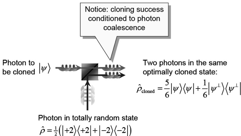
Figure 8. Pictorial illustration of the optimal quantum cloning based on the symmetrization method in a beam-splitter for the case of OAM-qubit-carrying photons.
