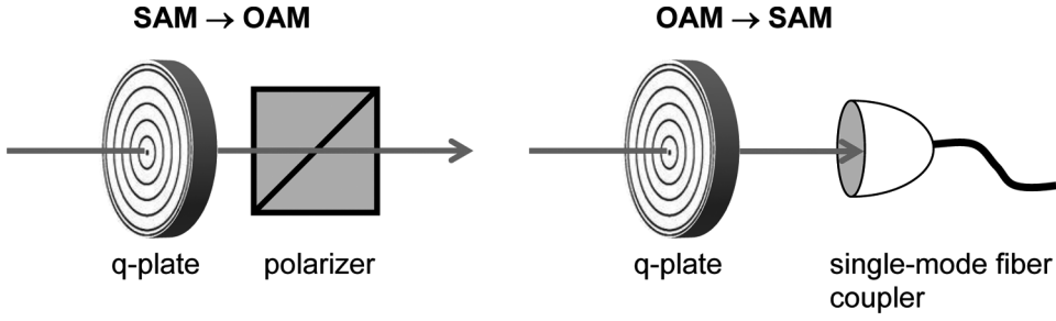
Figure 3. Pictorial representation of the simplest devices for the transfer of a qubit of quantum information from the polarization to the OAM (SAM → OAM) and vice versa (OAM → SAM).
